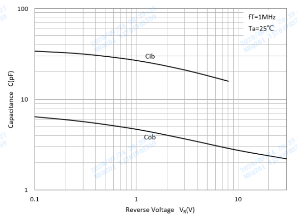
C_{ob}/C_{ib}-V_{CB}/V_{EB}
