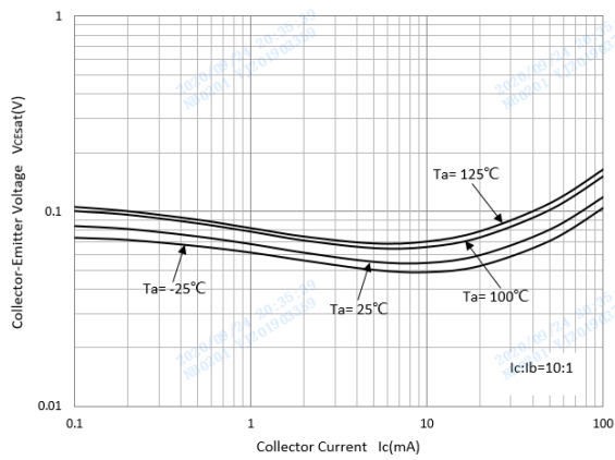
Collector-Emittor Saturation Voltage
